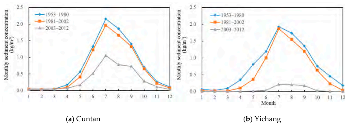
Figure 4. Impact of reservoirs on the monthly distribution of sediment concentration. Notes: the average monthly sediment concentration ( \text{kg}/\text{m}^3 ) was calculated using the average monthly sediment discharge ( \text{kg}/\text{s} ) divided by the average monthly flow discharge ( \text{m}^3/\text{s} ) according to the Code of Hydrologic Data Compilation [32].
